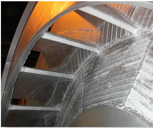
Cr-Carbide liners
