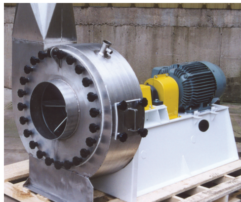
Stainless steel spray dryer dairy fan
